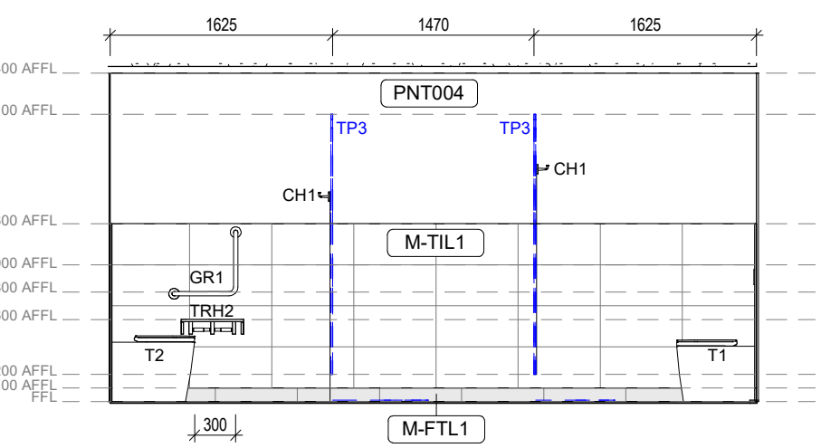
7 Game Over - Amenities - Female - Elevation 3 1:50
