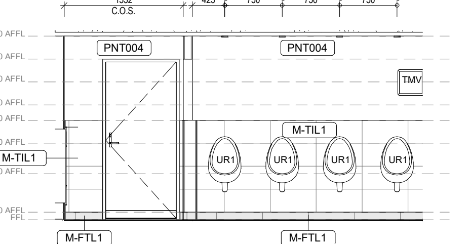
11 Game Over - Amenities - Male - Elevation 3 1:50
