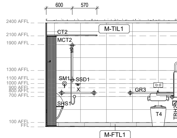
15 Game Over - Amenities - PWD - Elevation 1 1:50
