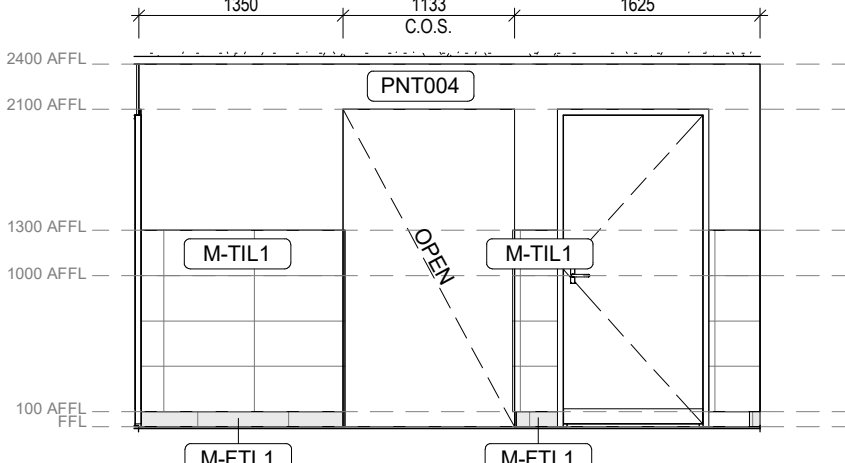
14 Game Over - Amenities - Male - Elevation 6 1:50
