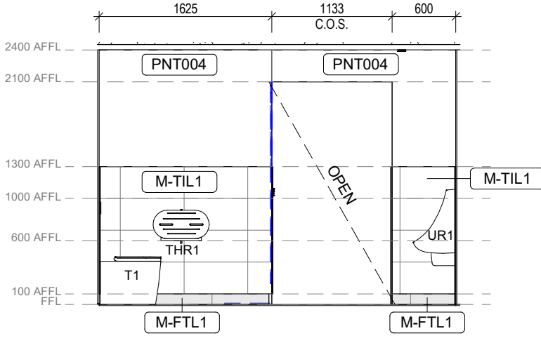
10 Game Over - Amenities - Male - Elevation 2 1:50
