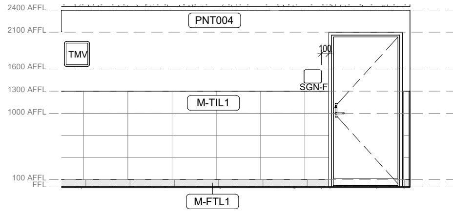
3 Game Over - Amenities - Corridor - Elevation 3 1:50
