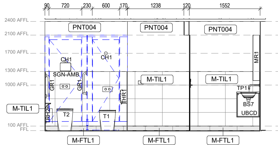
9 Game Over - Amenities - Male - Elevation 1 1:50
