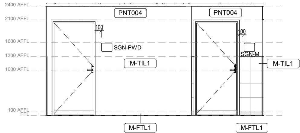
1 Game Over - Amenities - Corridor - Elevation 1 1:50
