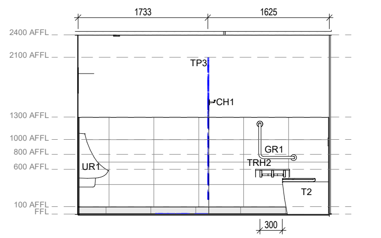
12 Game Over - Amenities - Male - Elevation 4 1:50
