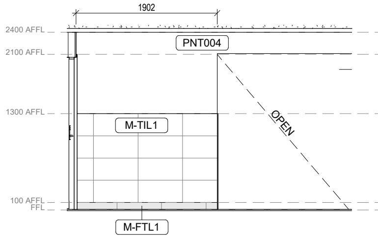
2 Game Over - Amenities - Corridor - Elevation 2 1:50
