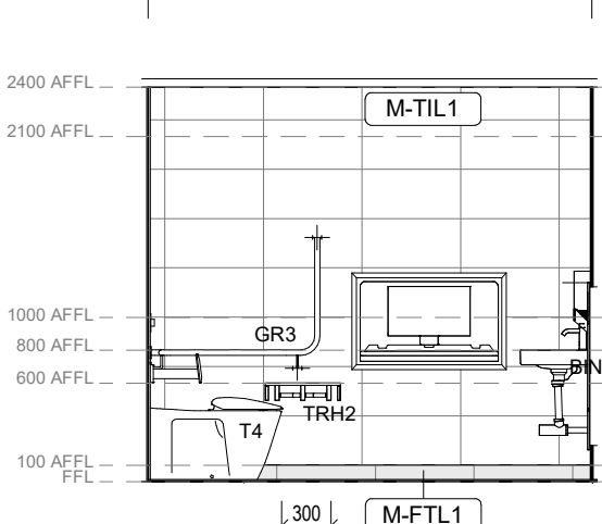
16 Game Over - Amenities - PWD - Elevation 2 1:50
