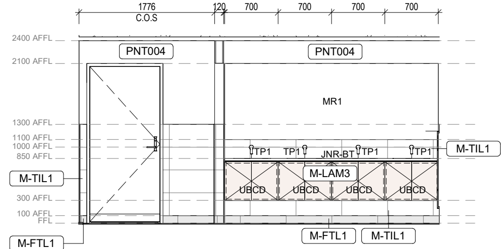
5 Game Over - Amenities - Female - Elevation 1 1:50
