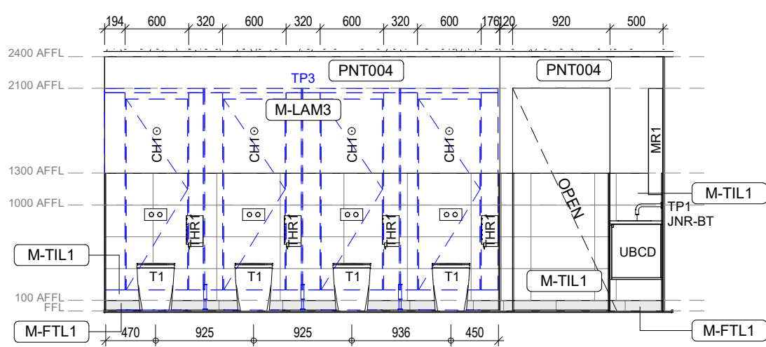
8 Game Over - Amenities - Female - Elevation 4 1:50
