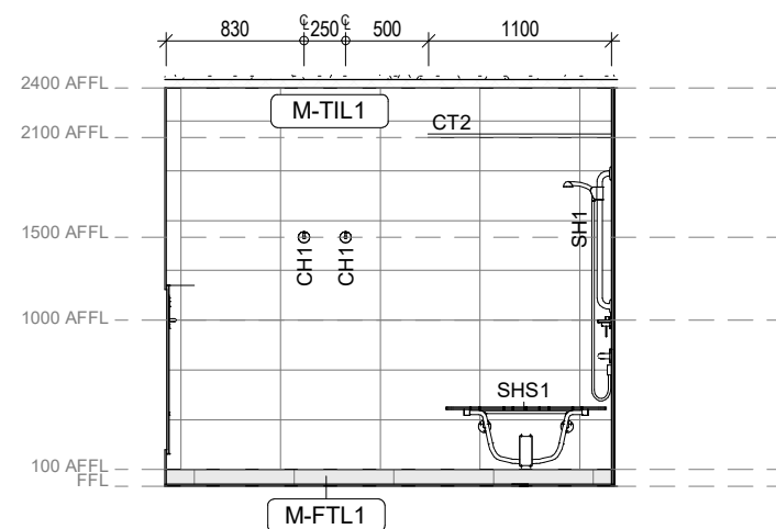
18 Game Over - Amenities - PWD - Elevation 4 1:50
