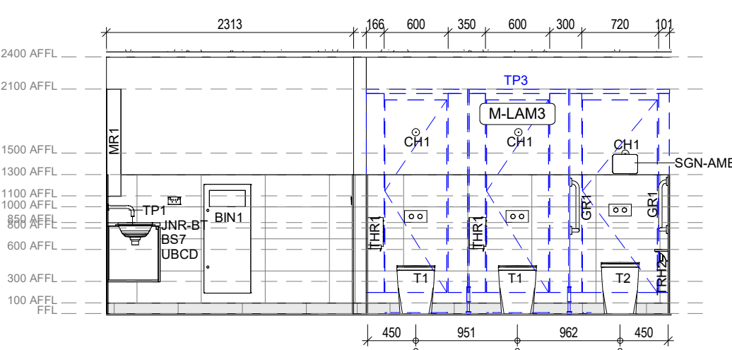
6 Game Over - Amenities - Female - Elevation 2 1:50
