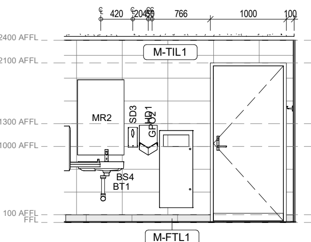
17 Game Over - Amenities - PWD - Elevation 3 1:50
